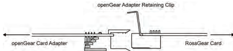
Figure 15. Disengaging the Cards
