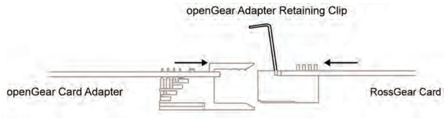
Figure 8. Mating the RossGear Card with the openGear Card Adapter
