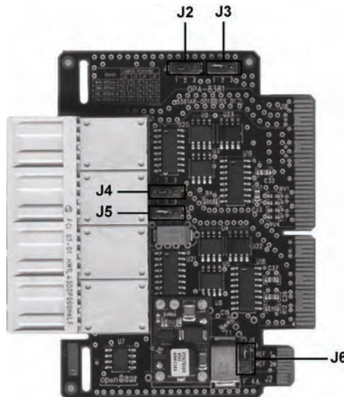
Figure 4. OPA-8381 — Jumper Locations
