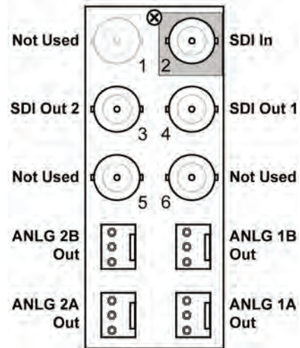
Figure 19. Cable Connections for the DMX-8554A-C
