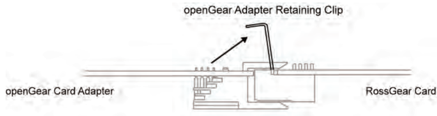
Figure 14. Positioning the openGear Adapter Retaining Clip – Side View
