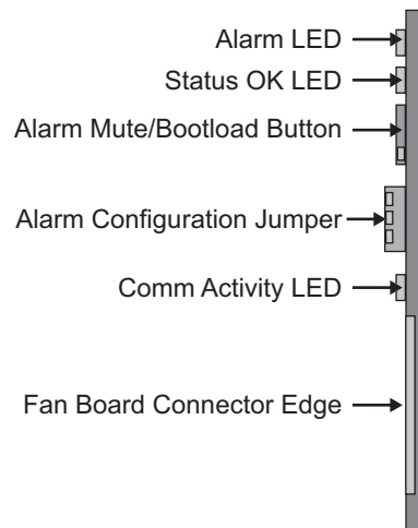
Figure 5.1 MFC-8310 Card-edge Controls
