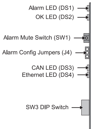
Figure 4.4 MFC-8320-N Card-edge Controls
