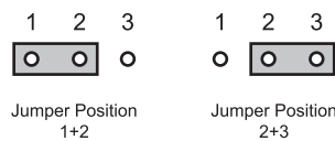
Figure 3.3 Alarm Config Jumper — Pin Positions
