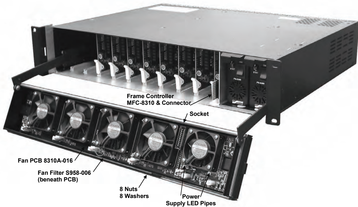
Figure 9. CFM-8310 Cooling Fan Module
