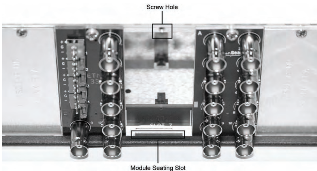
Figure 2.4 Rear Module Installation — DFR-8310 series frame
